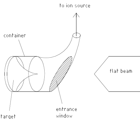
Fig. 3. Target container configuration for high power primary beam.
