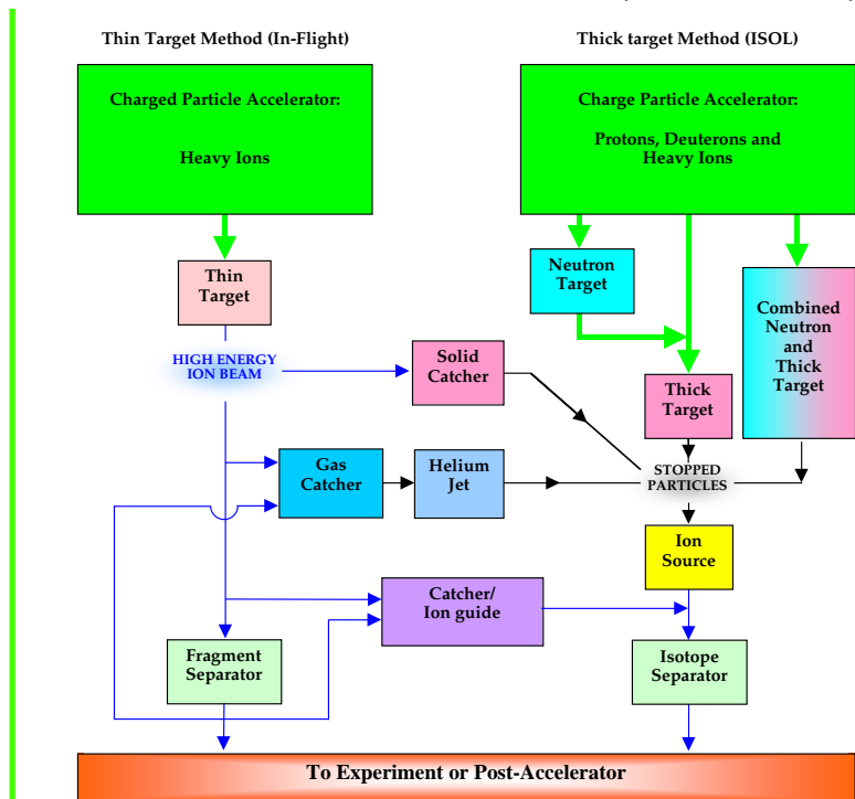
Figure 1. All potential RIB production methods with a heavy ion driver [ref. 4]. GANIL already developed and routinely uses most of the branches shown.
