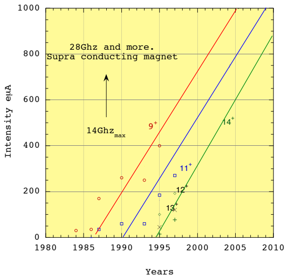
Fig. 5 : Evolution of the intensity of Ar during the last two decades [ref. 10]. The different lines indicate an extrapolation.
