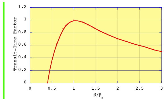
Fig 8 : Transit-time factor for a 2 gap cavity
