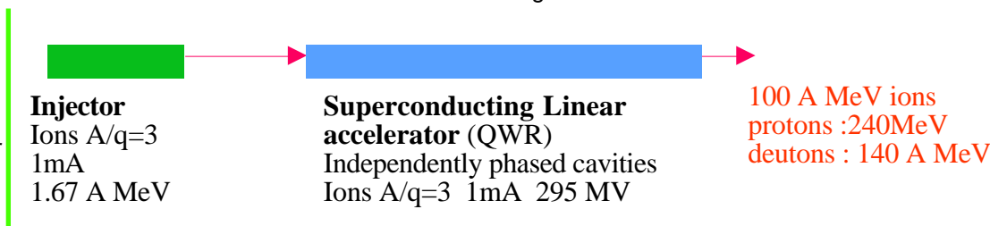
Fig. 6 : Schematic layout of the linear accelerator
