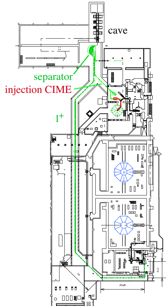
Figure VII.2 : Layout at the below ground level of the LINAG target-ion source cave and beam transport to the low-energy area, CIME and the C02 injection cyclotron.
