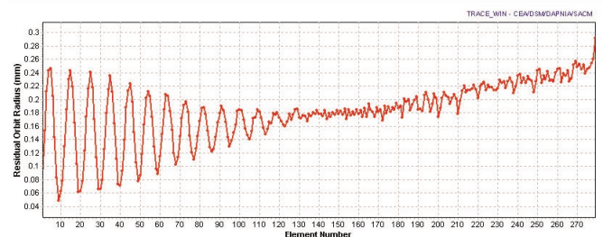
Figure IV.7 : Oscillation of the beam centroid along the proposed LINAG RFQ, with full error combination.
