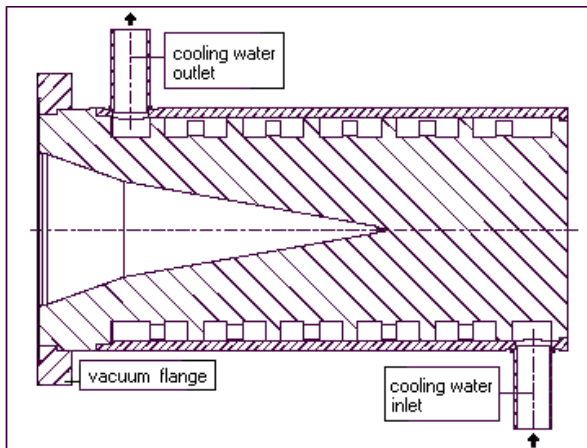
Figure 12 Beam Dump Principle (scheme from ELBE project)
