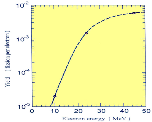
Figure 3 Fission yield vs electron energy
